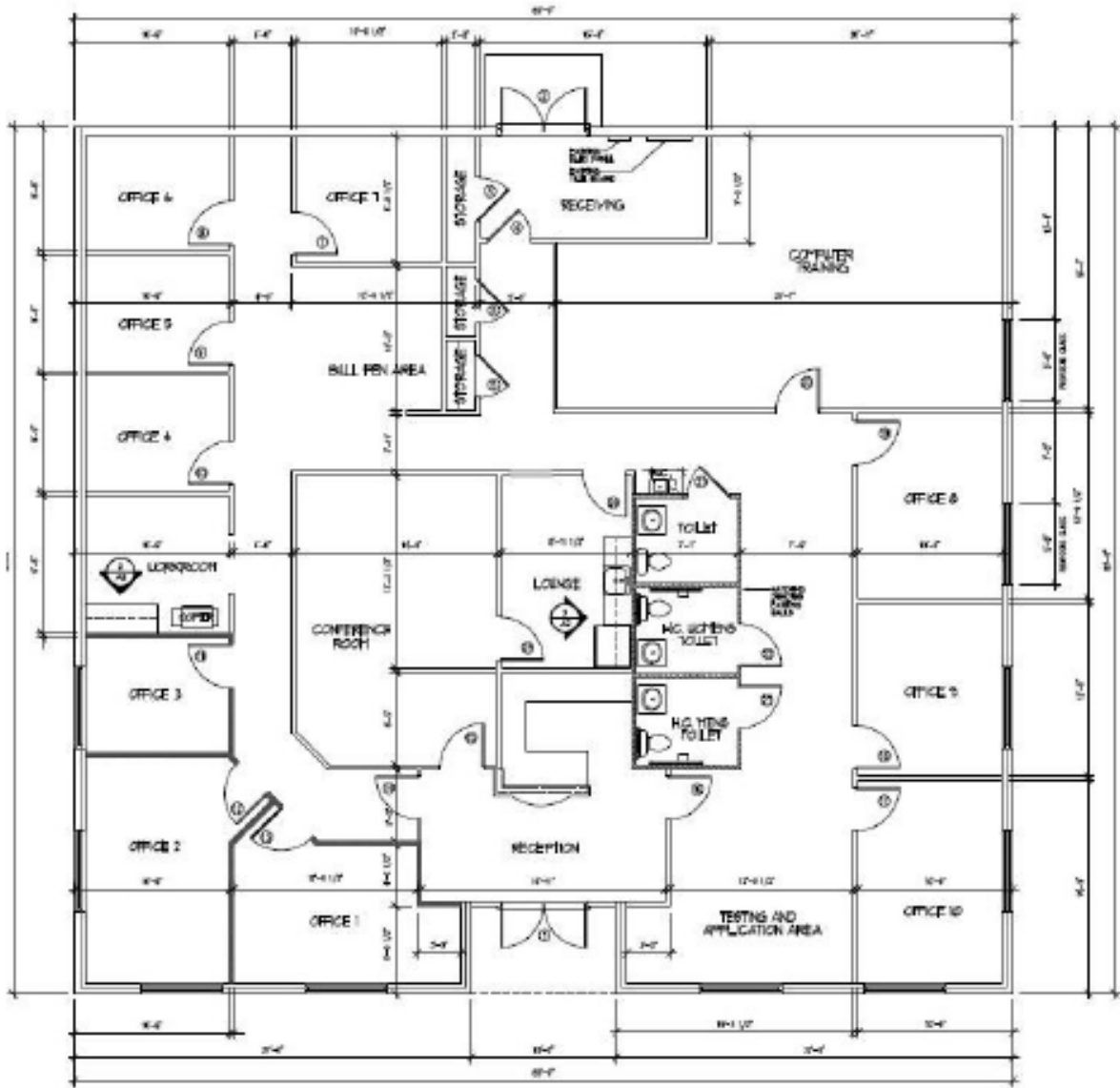
1 FLOOR PLAN 1/8" = 1'
