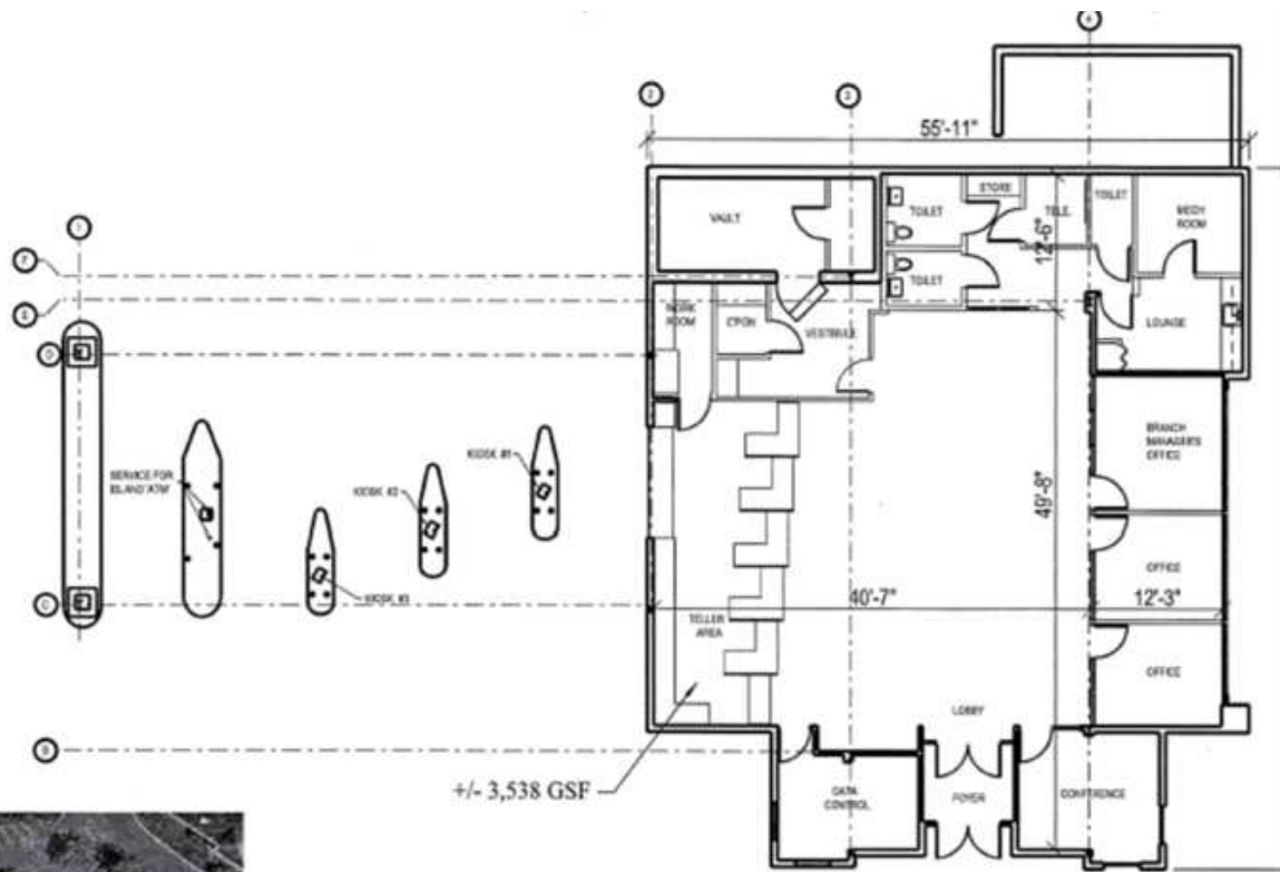
FLOOR PLAN - SCALE: 1/16" = 1'-0"
